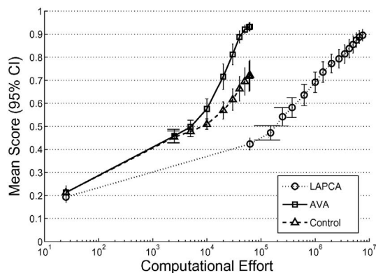
Fig. 6. Mean performance ( \pm 95\% C.I., 30 runs) against computational effort (number of network evaluations, presented on a log-scale) of coevolved sorting networks. AVA significantly outperforms the control. In contrast, LAPCA requires an order of magnitude more effort to reach equivalent performance.
