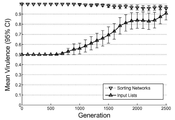
Fig. 4. Mean virulence ( \pm 95\% C.I.) of coevolved sorting networks and input lists over 30 runs. Sorting networks initially have a high virulence of 1.0, with input lists having low virulence of 0.5. Over time the virulence of input lists gradually increases as the bias between populations falls.
